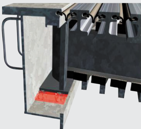
Fuse link for transversal seismic movements
